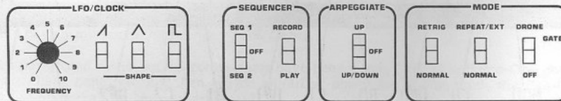
Figure 1-1 KEYBOARD CONTROLS
