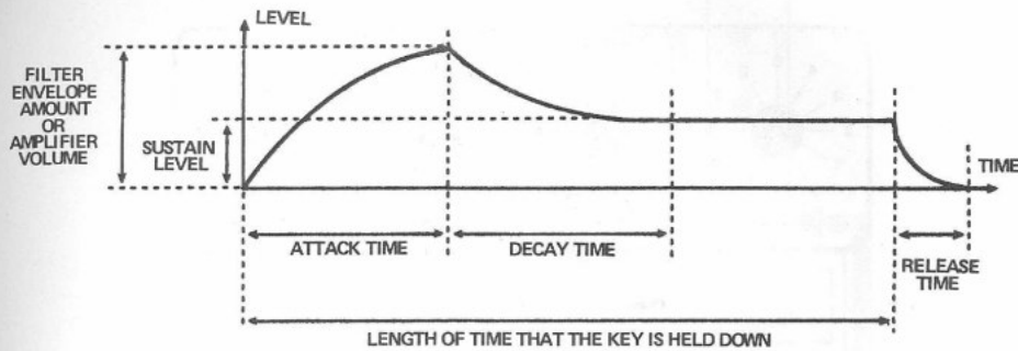
Figure 2-6 ENVELOPE
