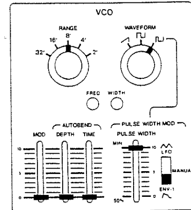
4 ENVELOPE MODULATION OF PULSE WAVE
