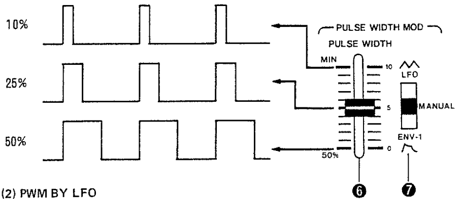
(2) PWM BY LFO
