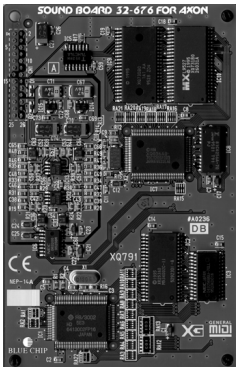
Sound card SB-676 GM / XG sound card with 480 sounds, 11 reverbs, 41 effects..
